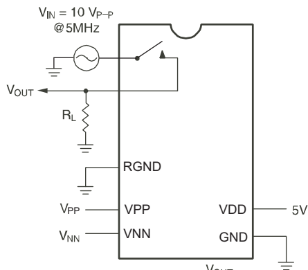
OFF Isolation
