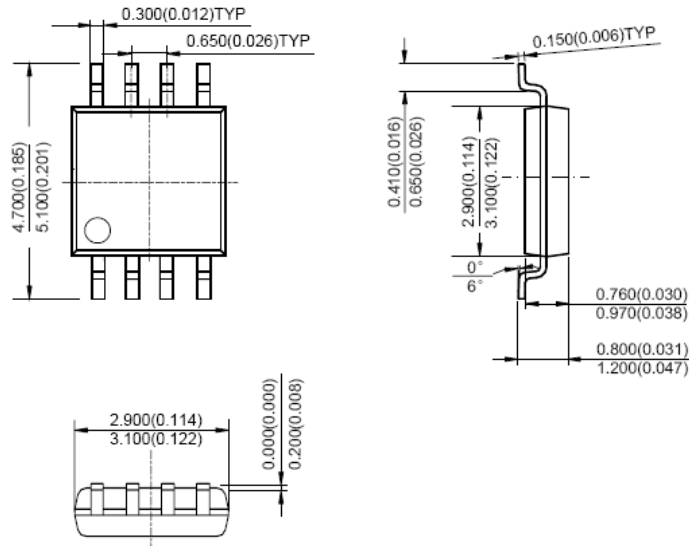
MSOP-8
