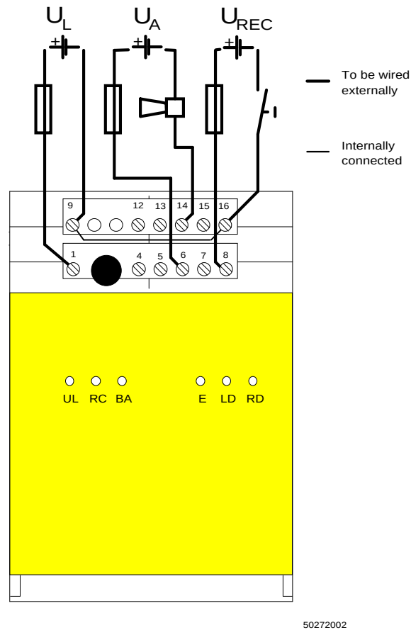
Fig. 3: Connection of the supply voltage
