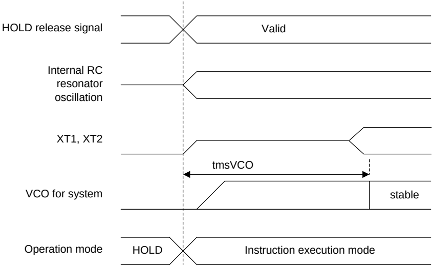
HOLD release signal and oscillation stabilizing time Figure 2 Oscillation Stabilizing Time
