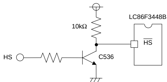
Figure 5 Recommended Interface Circuit
