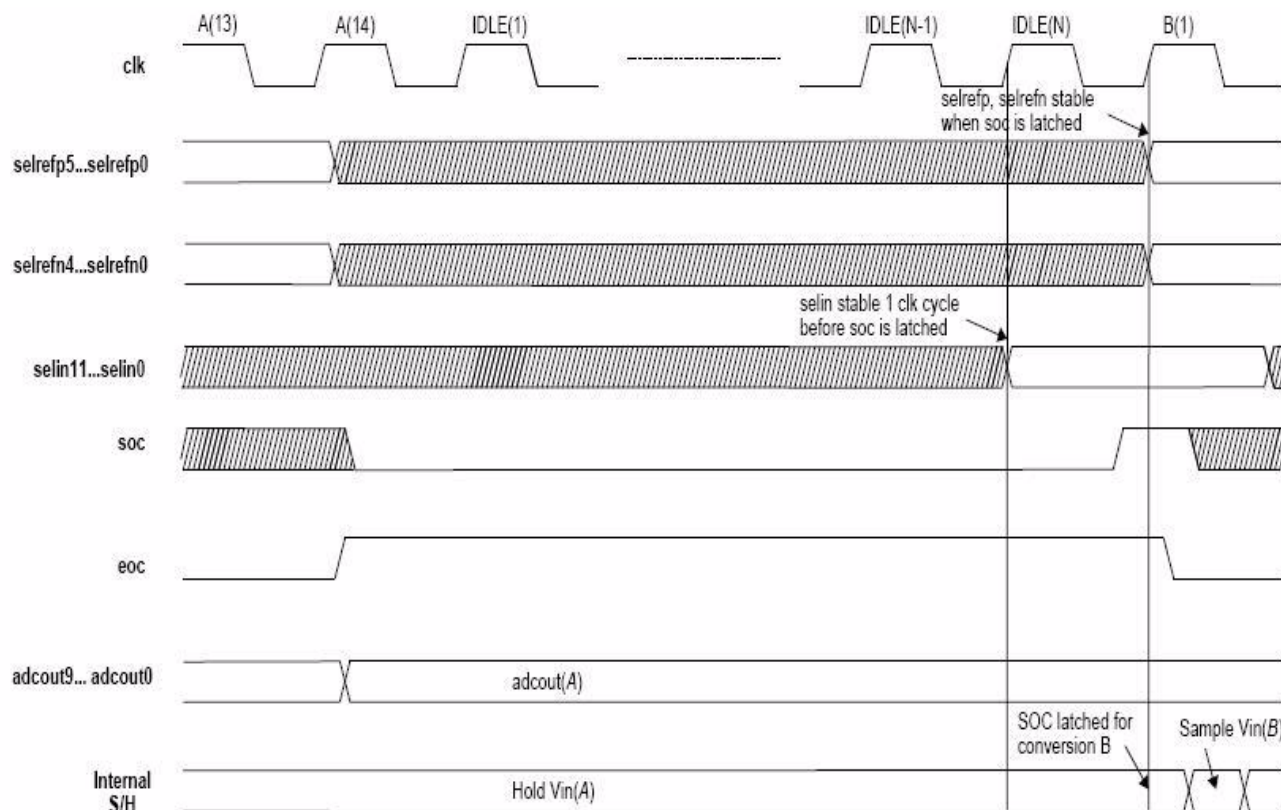
Figure 84. ADC Usage with Idle Cycles Between Conversions
