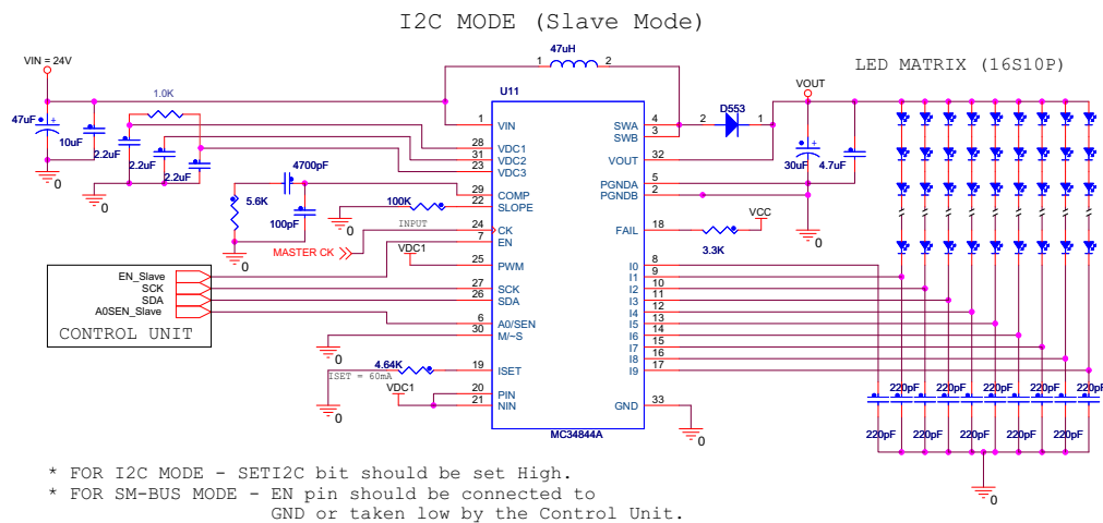
Figure 30. I 2 C (Slave Mode)
