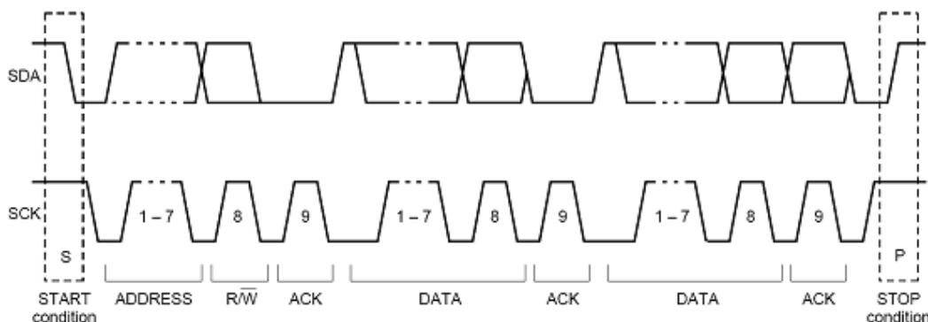
Figure 26. A Complete Data Transfer
