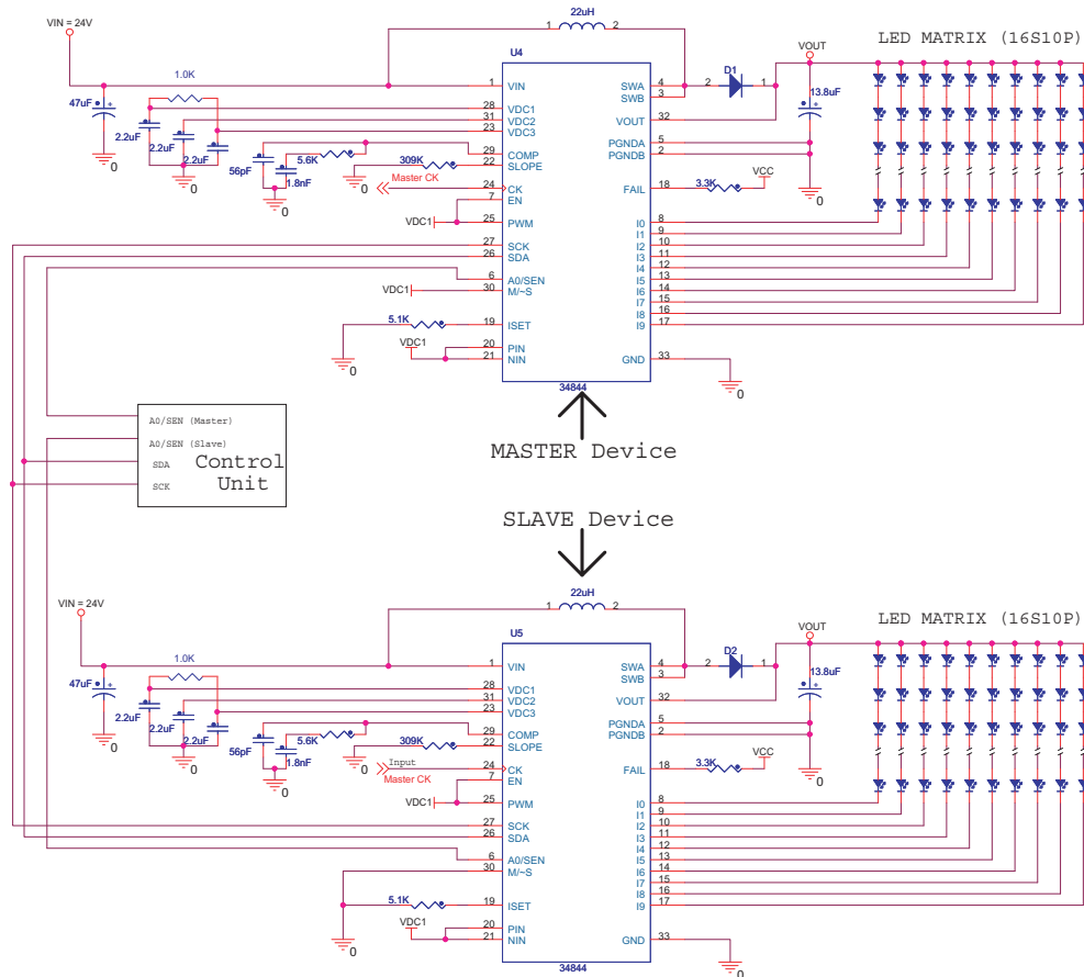
Figure 22. Master - Slave Connection
