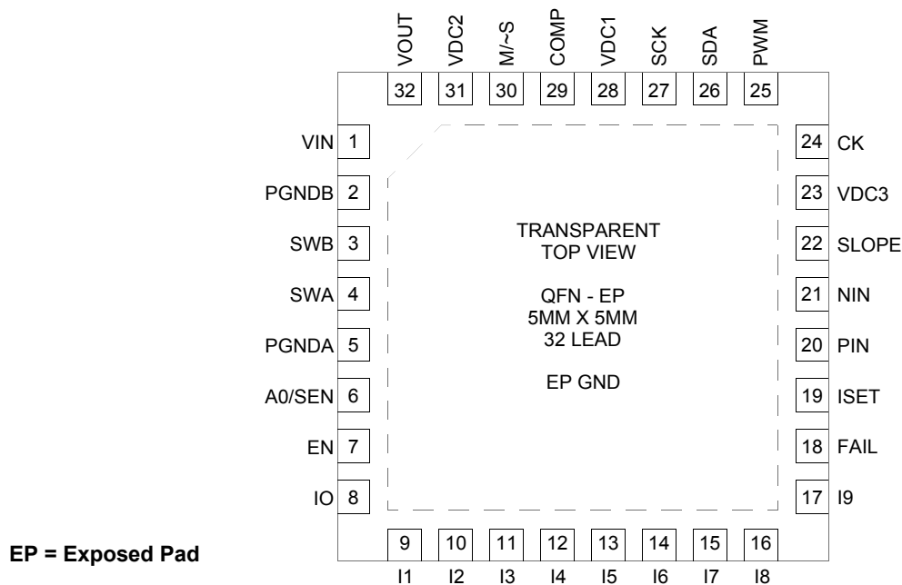
Figure 24. 34844A Pin Connections
