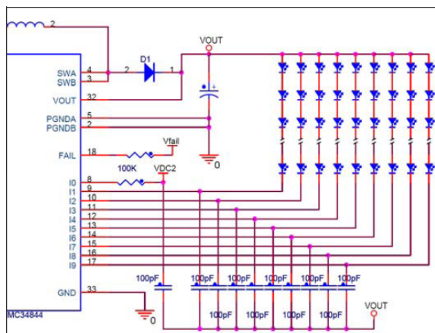
Figure 6. Single Channel Disconnect Circuit.
