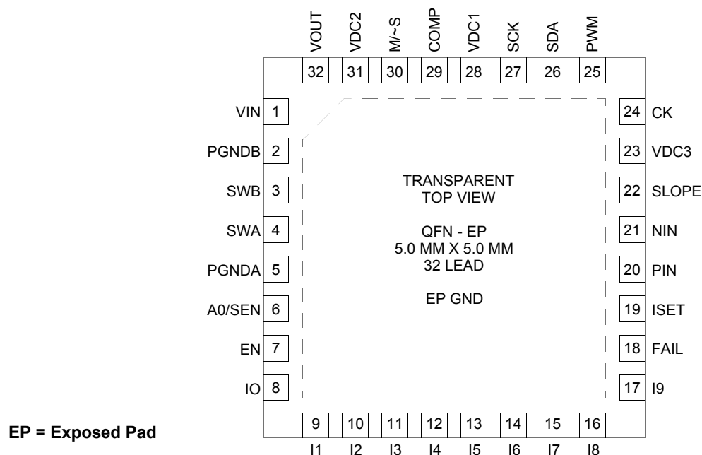
Figure 4. 34844 Pin Connections
