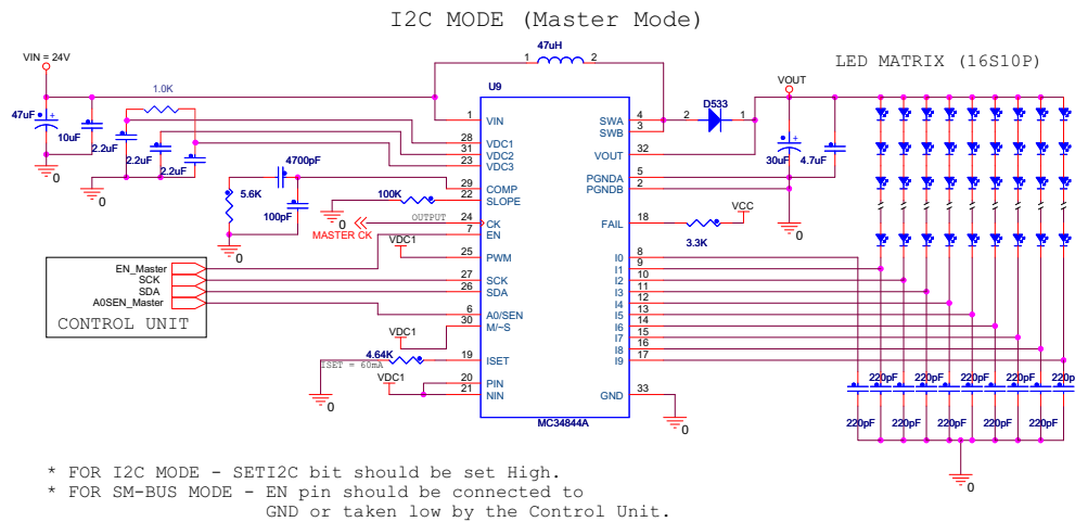
Figure 29. I 2 C (Master Mode)
