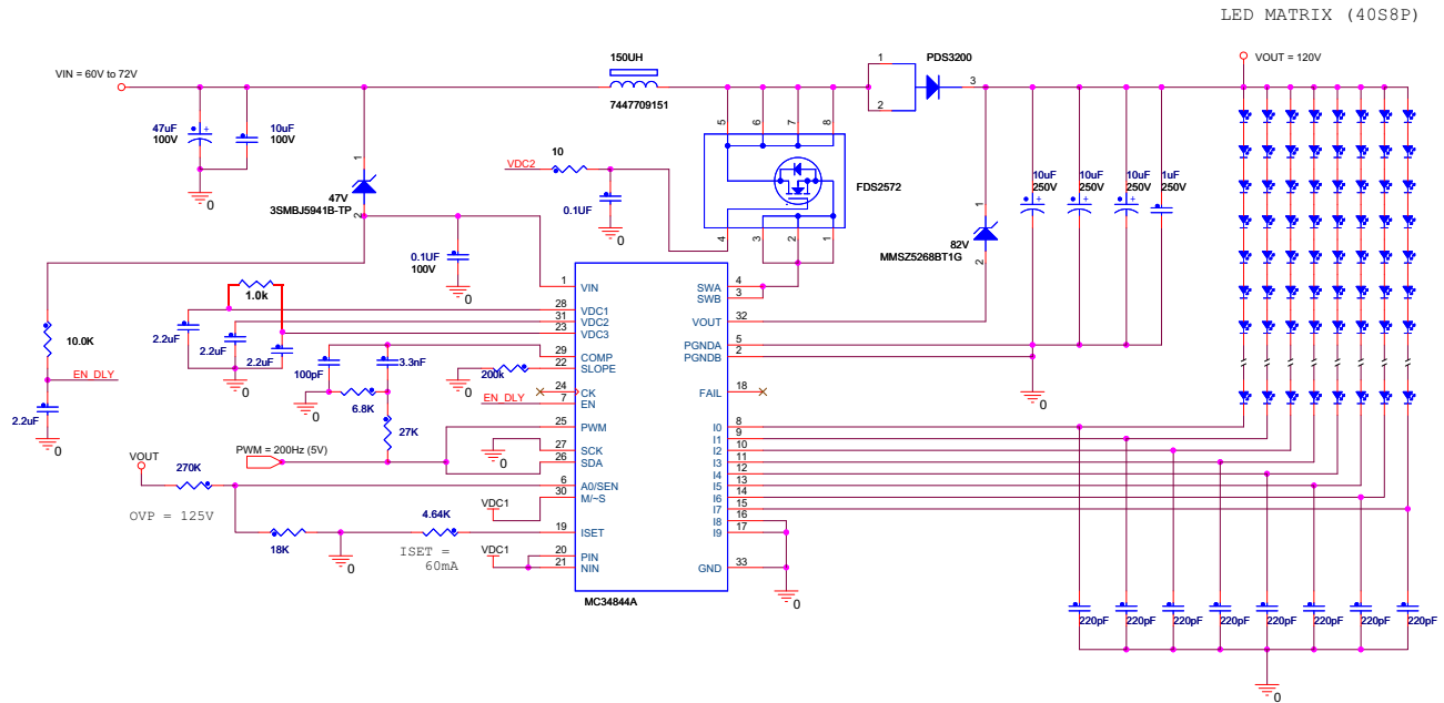
Figure 31. HIGH VOUT application (Manual Mode)
