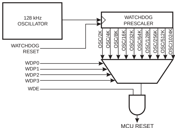
Figure 20. Watchdog Timer
