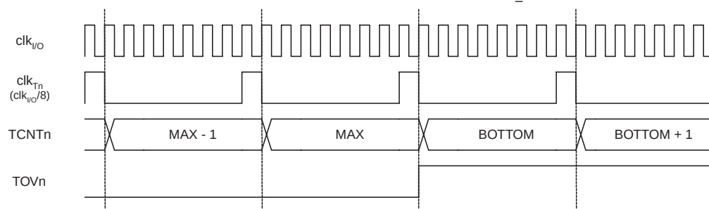
Figure 34. Timer/Counter Timing Diagram, with Prescaler ( f_{clk\_I/O}/8 )
