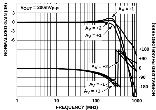
FIGURE 4. FREQUENCY RESPONSE
