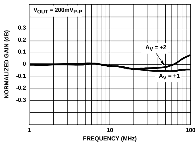
FIGURE 6. GAIN FLATNESS
