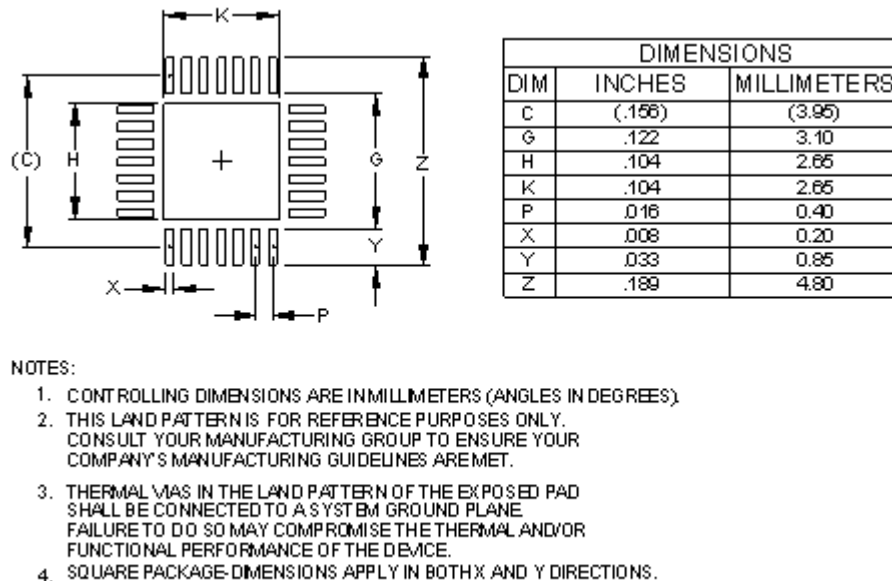
Figure 67 Land Pattern
