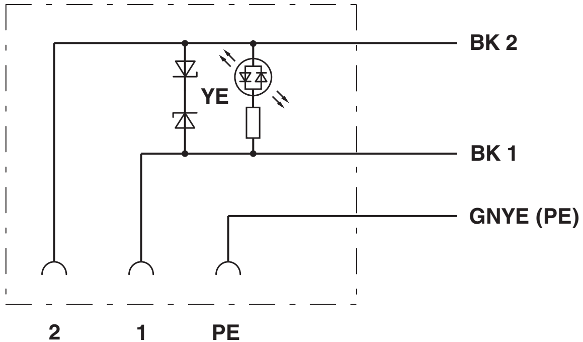
Circuit diagram
