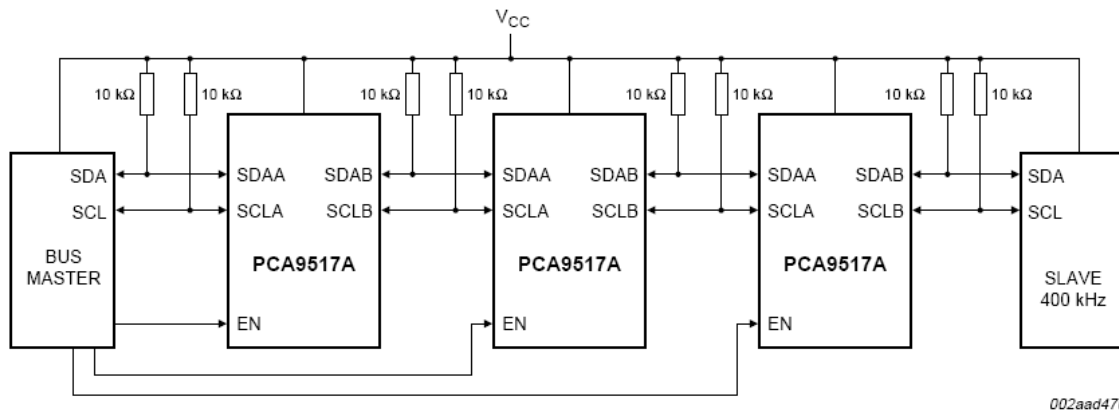
Figure 7. Typical Series Application
