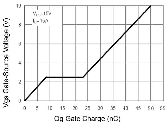
Figure 11 Gate Charge
