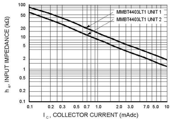
Figure 11. Input Impedance
