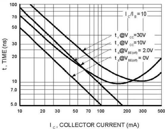
Figure 5. Turn-On Time
