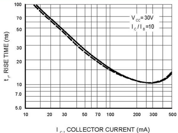
Figure 6. Rise Time
