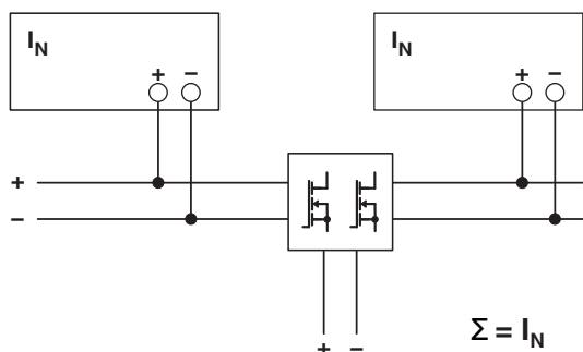
Figure 44 Schematic diagram, redundant operation with QUINT S-ORING
