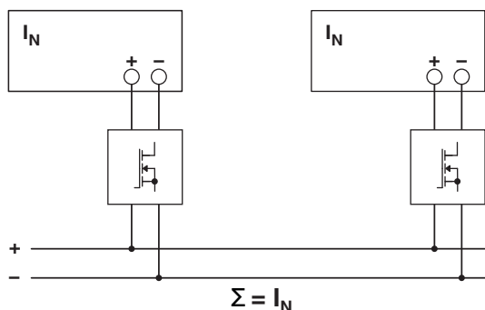
Figure 44 Schematic diagram, redundant operation with QUINT S-ORING
