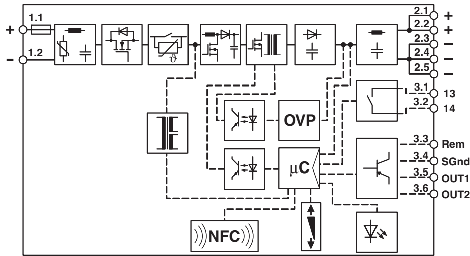
Figure 6 Block diagram
