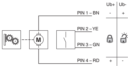
Block diagram of the locking actuator
