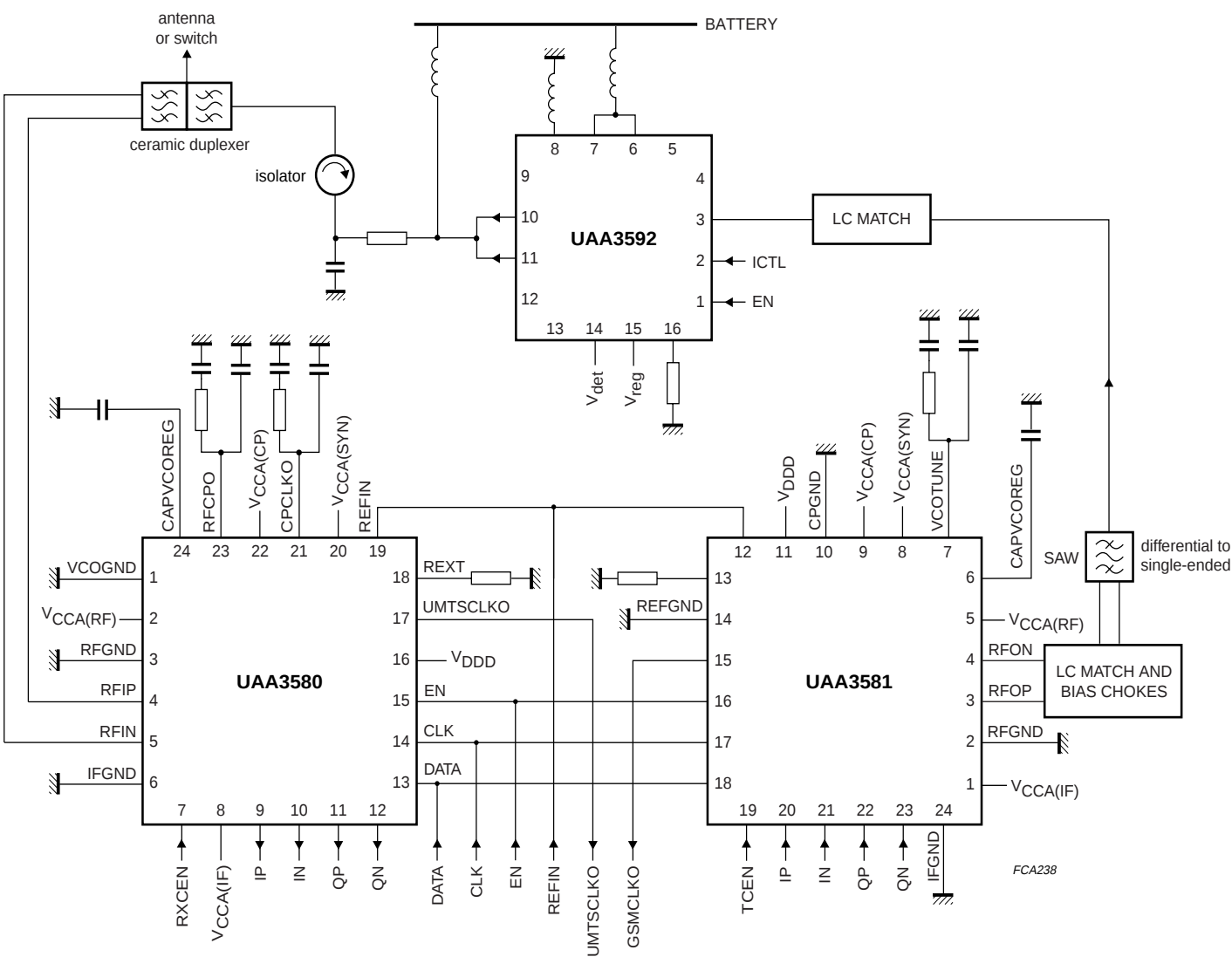
Fig.4 Application diagram.
