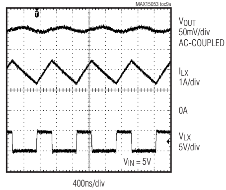
SWITCHING WAVEFORMS ( I_{OUT} = 2A )
