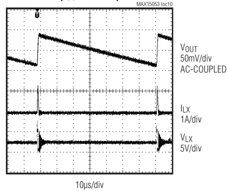
SWITCHING WAVEFORM IN SKIP MODE ( I_{OUT} = 10mA )
