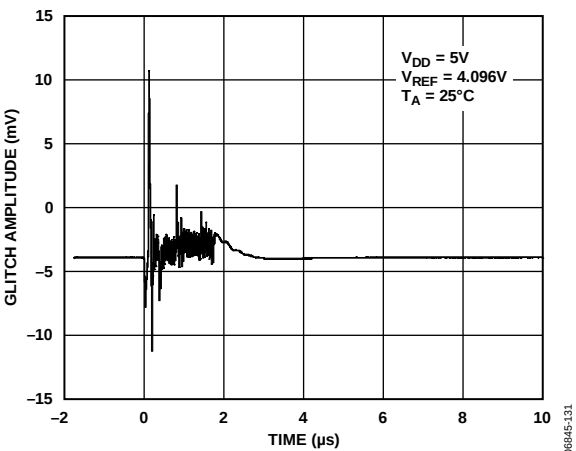
Figure 31. Digital Crosstalk
