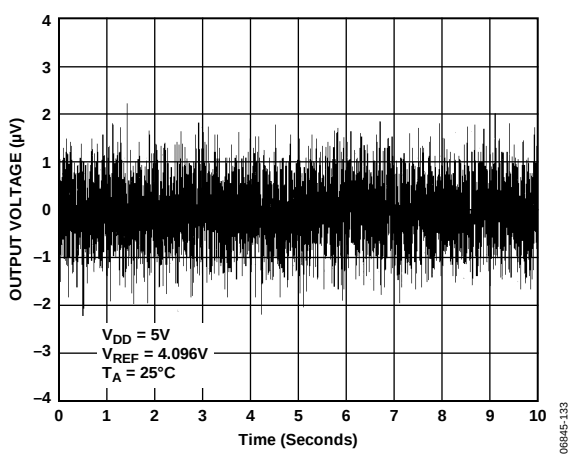
Figure 33. 1/f Noise
