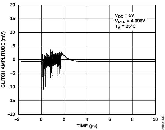
Figure 32. DAC-to-DAC Crosstalk
