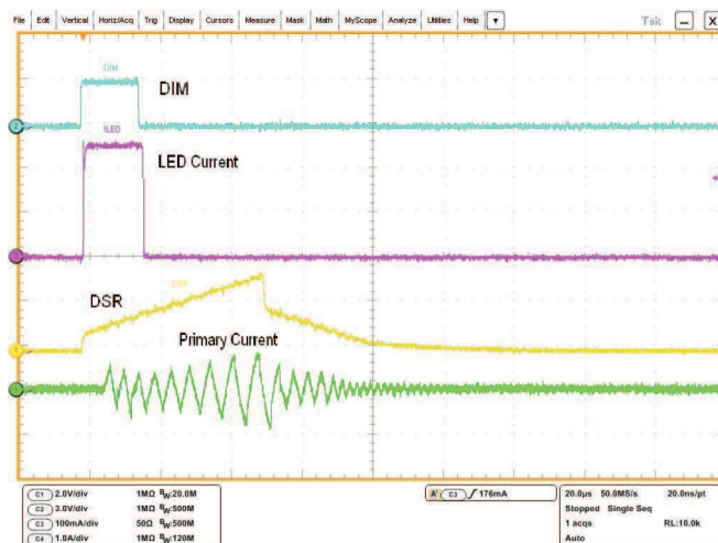
Figure 27. 0.5% DIM duty-cycle
