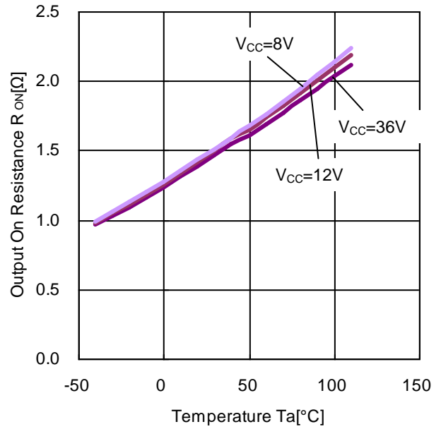
Figure 24. Output On Resistance vs Temperature (Output ON Resistance High Side, I_o=0.8A )
