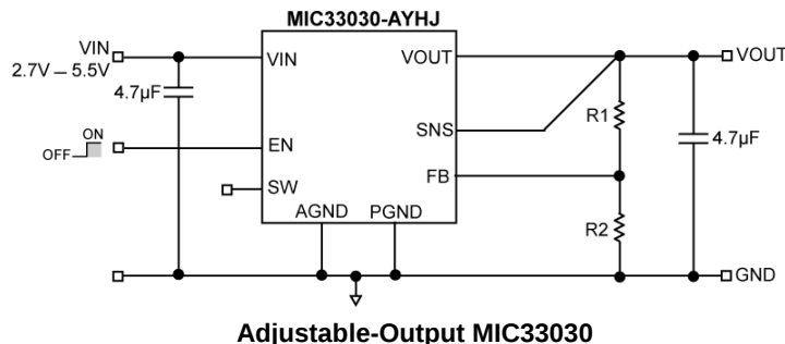
Adjustable-Output MIC33030
