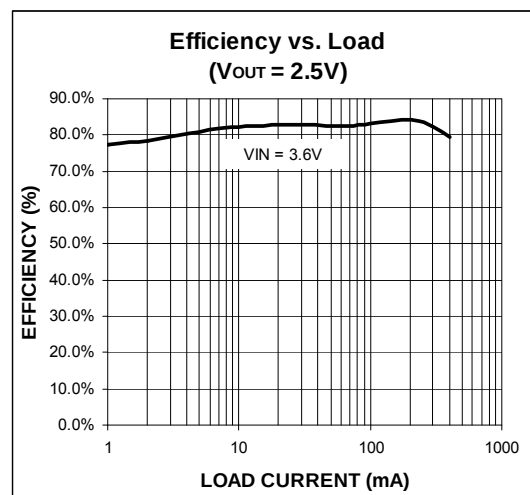
Figure 2. Efficiency under Load
