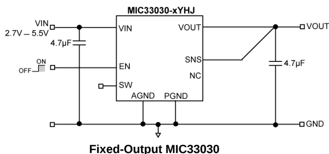
Fixed-Output MIC33030
