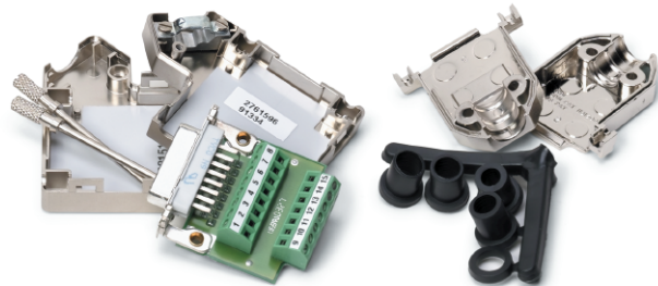
Figure 7. NI 9935 15-Pin D-Sub Connector Kit with Strain Relief and D-Sub Shell
