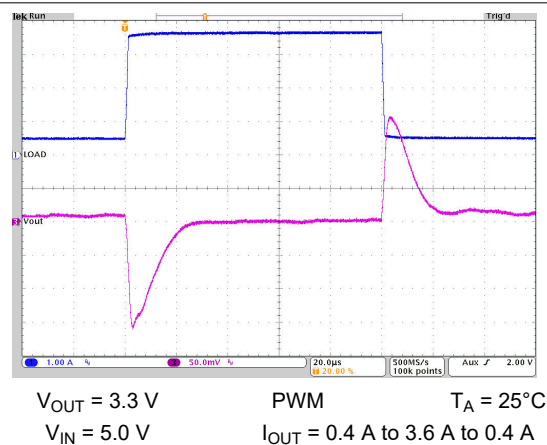
图 10-23. Load Transient Response
