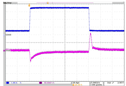
图 10-27. Load Transient Response
