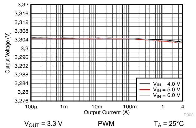
图 10-13. Output Voltage versus Output Current
