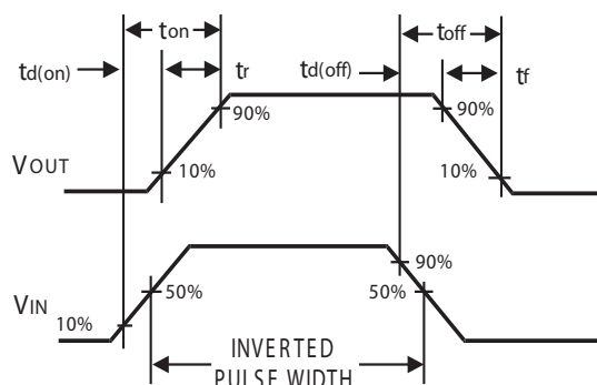
FIG.12 Switching Waveforms
