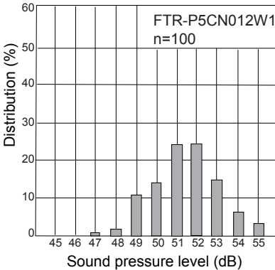
Distribution of sound pressure (with diode)
