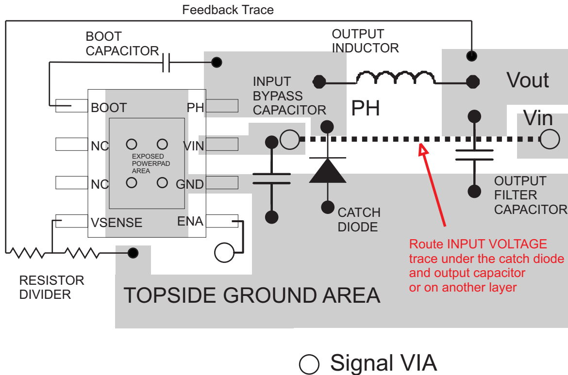
Figure 9. Design Layout
