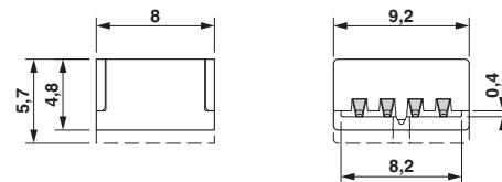
Dimensional drawing
