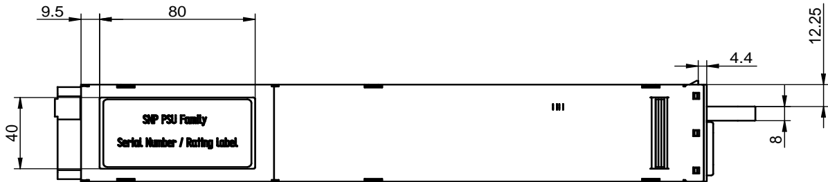
Figure 24. Side View 1
