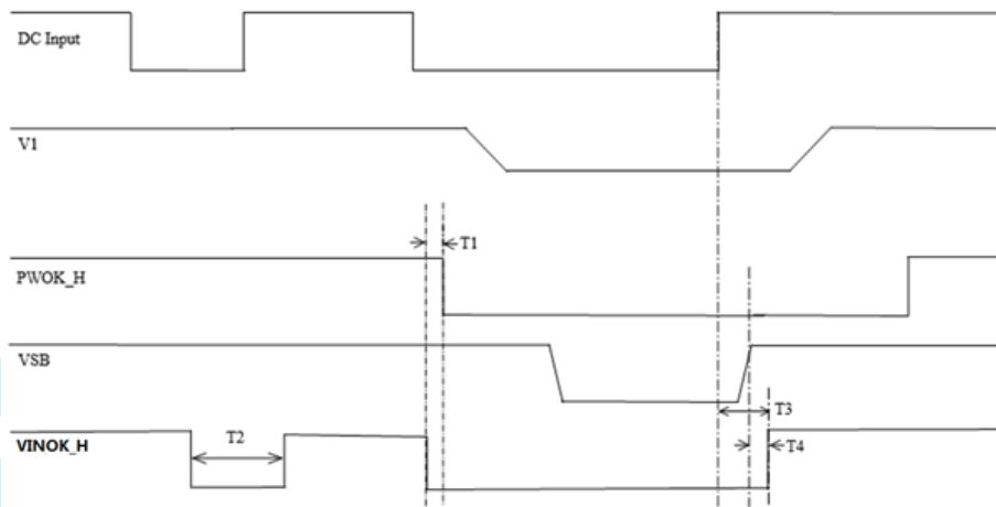
Figure 12. VINOK_H Timing
