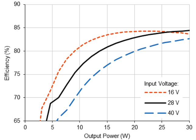
4.1.2 VHR30-2812D Efficiency (%) vs. Output Power (W)
