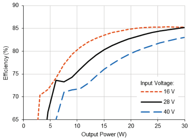
4.1.3 VHR30-2815D Efficiency (%) vs. Output Power (W)
