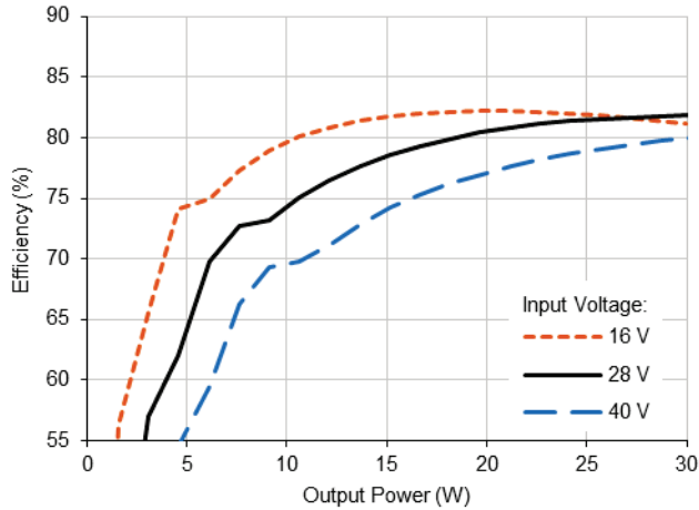
4.1.1 VHR30-2805D Efficiency (%) vs. Output Power (W)
