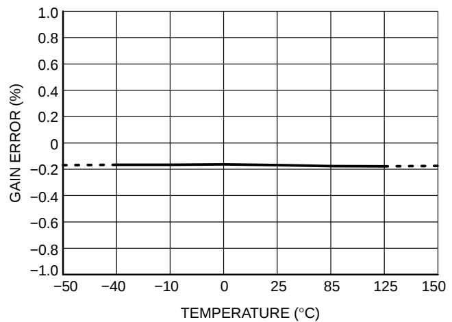
Figure 7. Gain Error vs. Temperature
