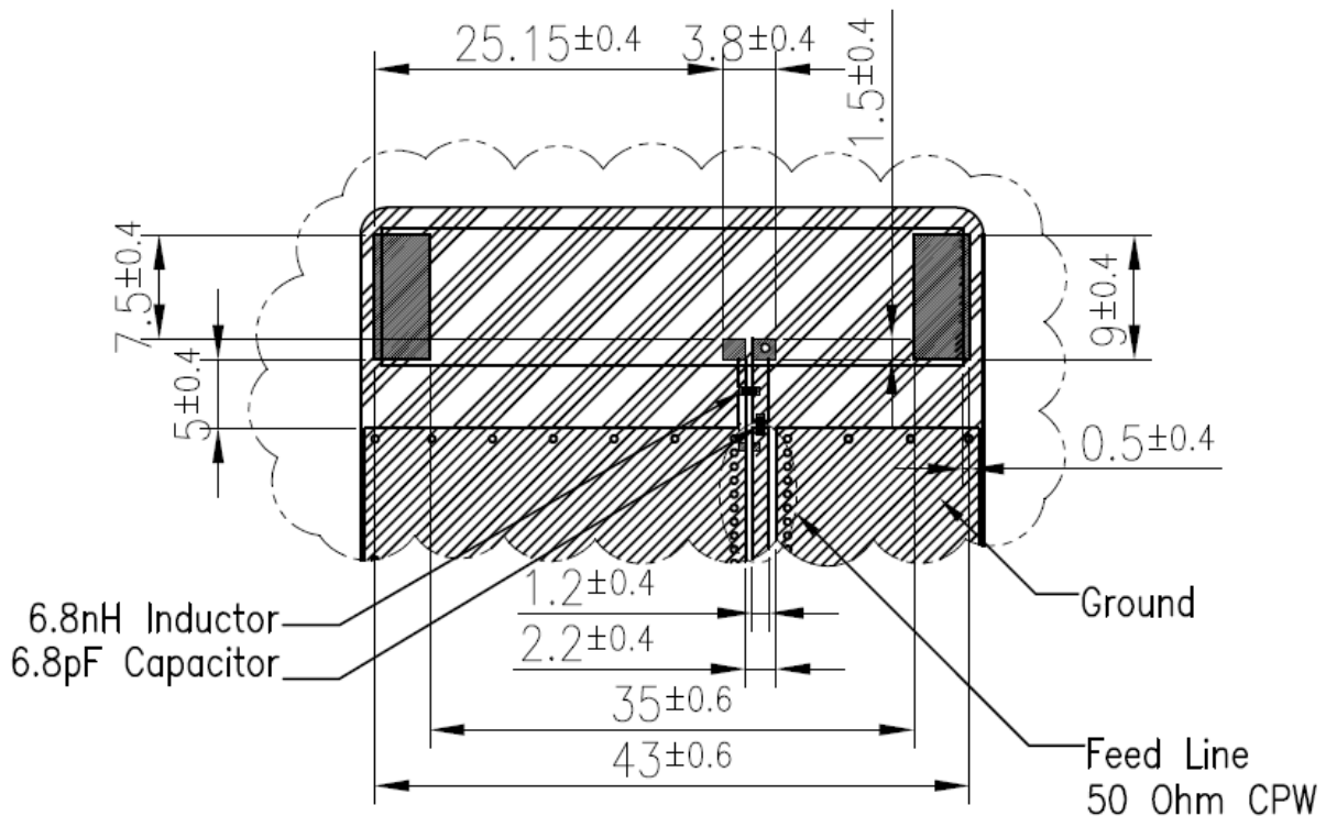
PCB Footprint
