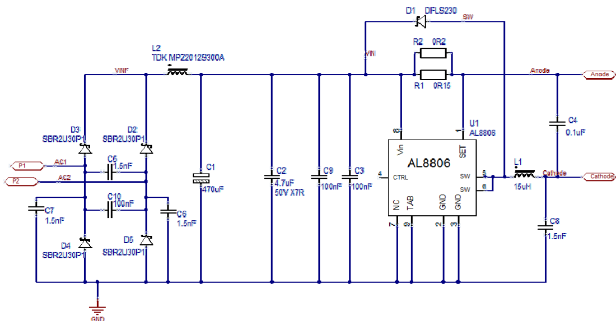
Figure 7. MR16 Schematic
