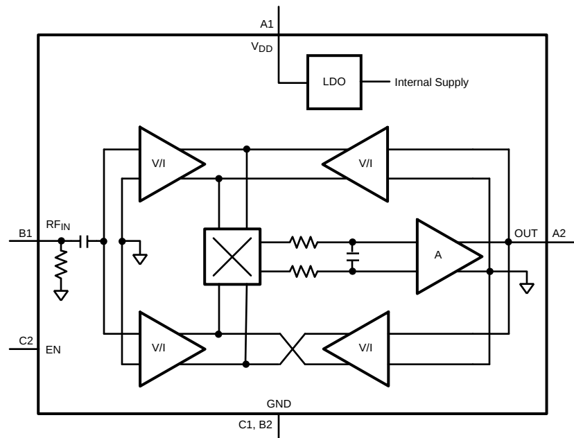
Figure 4. LMH2120
