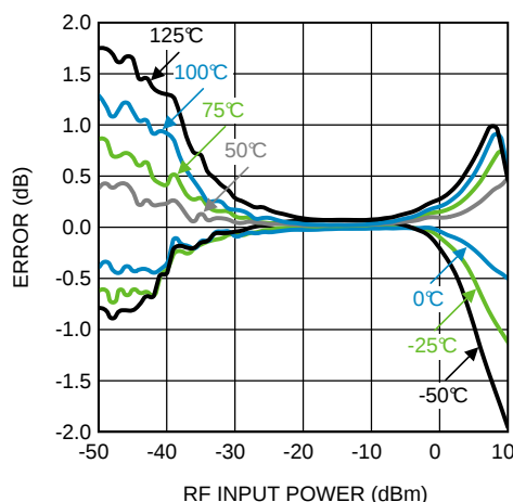
Figure 69. Temperature Variation vs. RF Input Power at 1900 MHz
