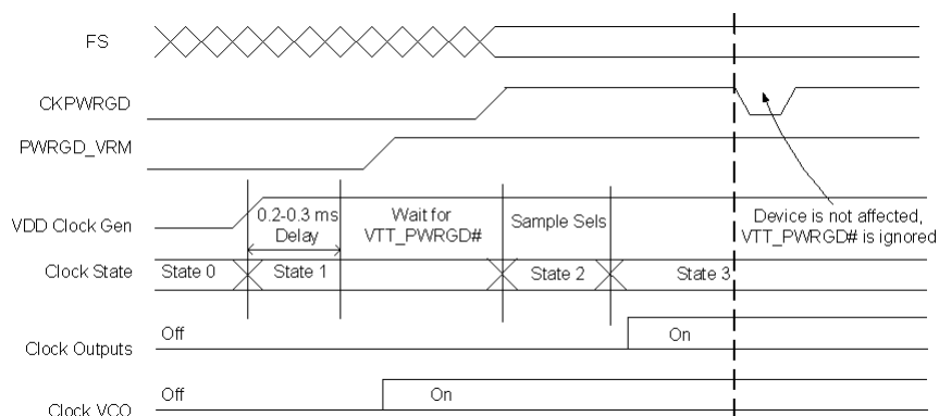
Figure 5. CKPWGRD Timing Diagram
