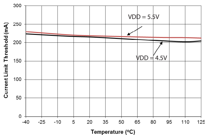
3.3V LDO Current Limit
