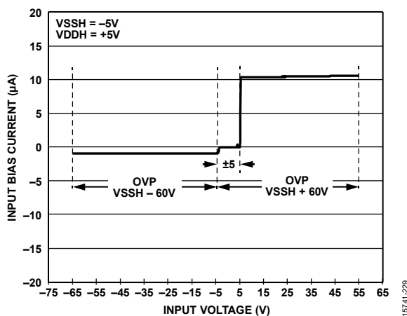
Figure 36. Input Overvoltage Performance, V_{DDH}/V_{SSH} = \pm 5 V
