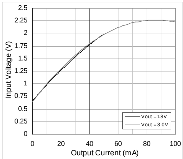
Figure 13. Startup Voltage vs. Output Current
