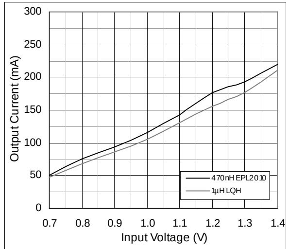
Figure 9. I_{OUT} vs. V_{IN} ; V_{OUT} = 1.8V
