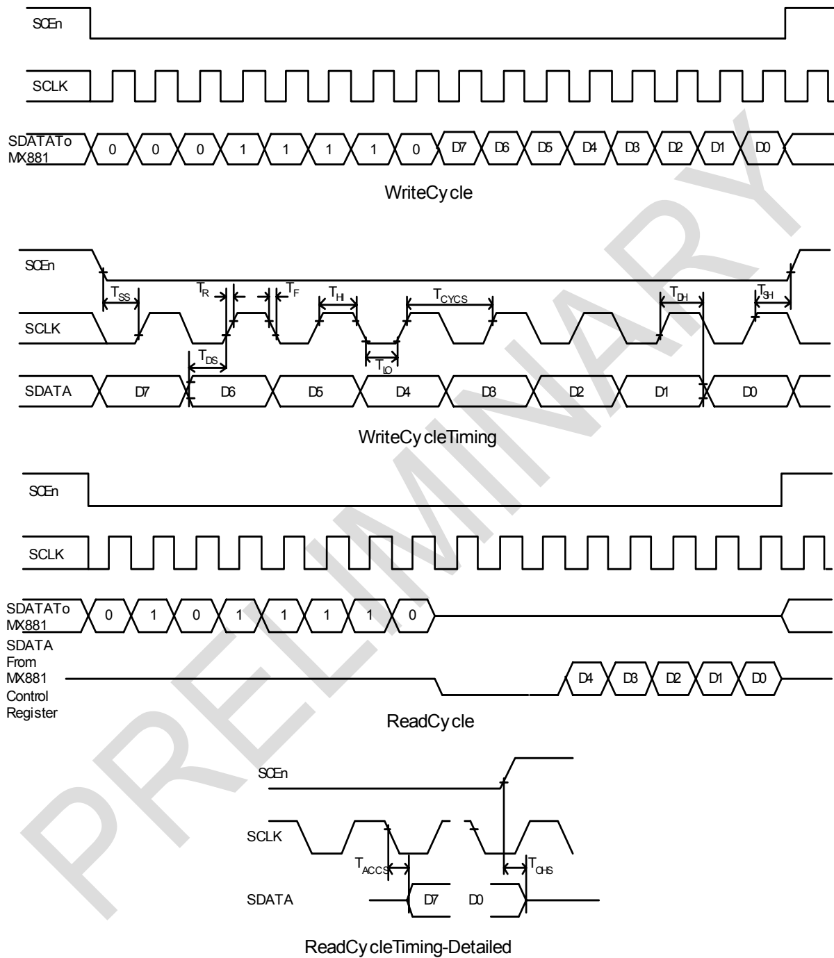
Figure 3 – 3-WIRE SPI
