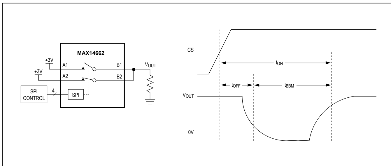
Figure 2. Turn-On/Turn-Off/Break-Before-Make
