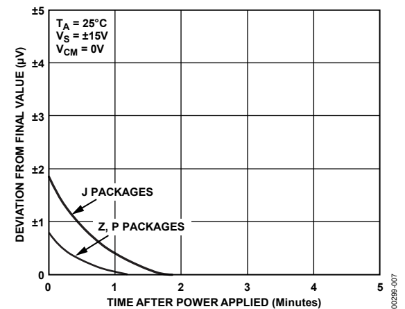
Figure 7. Input Offset Voltage Warmup Drift
