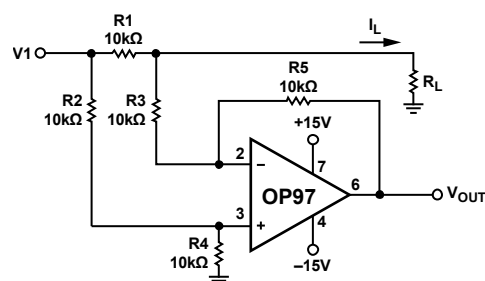
Figure 36. Current Monitor
