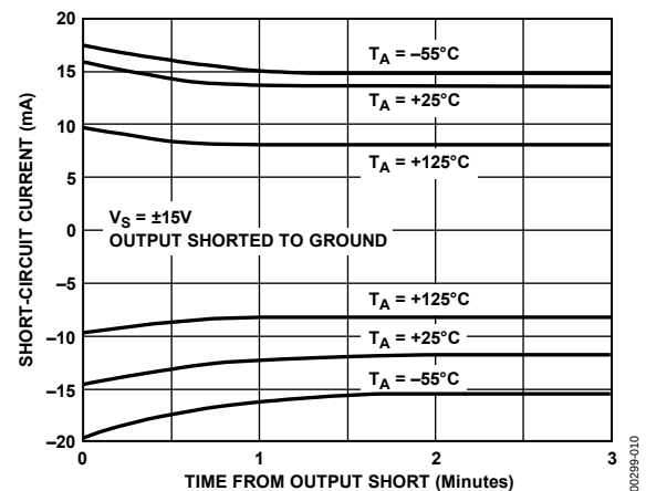
Figure 10. Short-Circuit Current vs. Time, Temperature
