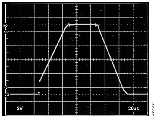
Figure 32. Large Signal Transient Response ( A_{VCL} = 1 )
