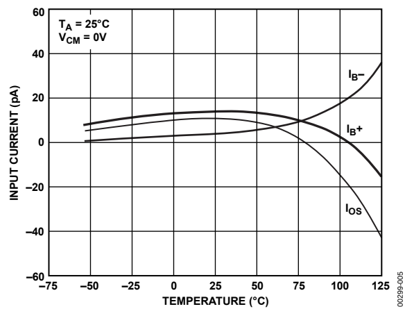
Figure 5. Input Bias, Offset Current vs. Temperature
