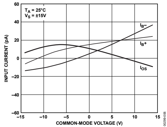
Figure 6. Input Bias, Offset Current vs. Common-Mode Voltage
