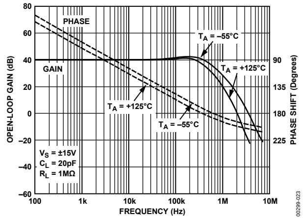
Figure 23. Open-Loop Gain, Phase vs. Frequency ( C_{OC} = 100 pF)
