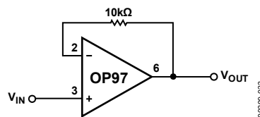
Figure 33. Unity-Gain Follower
