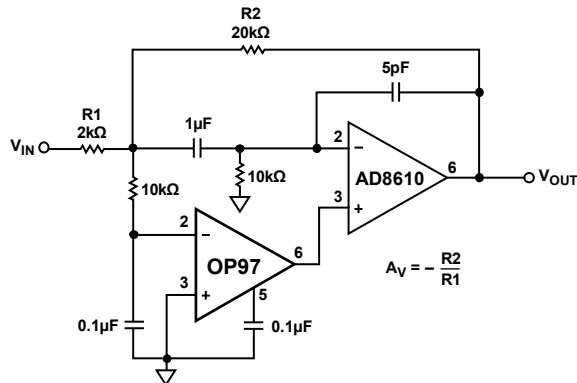
Figure 39. Combination High Speed, Precision Amplifier
