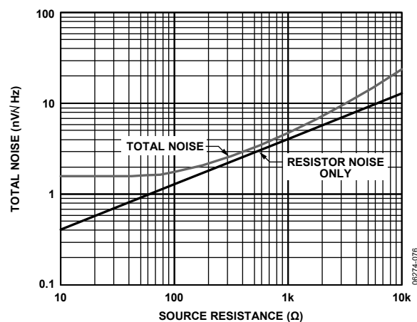
Figure 58. Noise vs. Source Resistance
