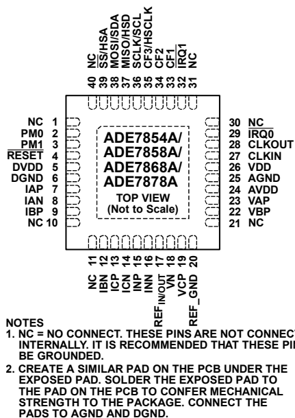
Figure 9. Pin Configuration
