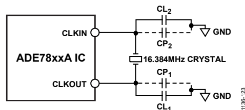
Figure 90. Crystal Circuit
