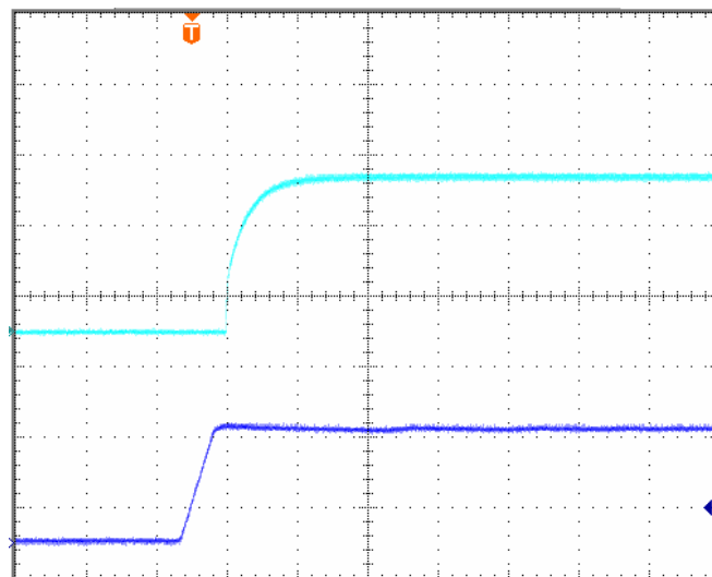
Figure 7: Turn-on transient at full rated load current (10 ms/div). Top Trace: Vout; 1.5V/div; Bottom Trace: input voltage: 30V/div.
