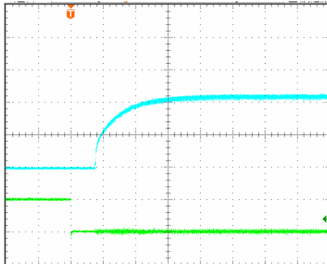
Figure 5: Turn-on transient at full rated load current (4 ms/div). Top Trace: Vout; 1.5V/div; Bottom Trace: ON/OFF input: 5V/div.
