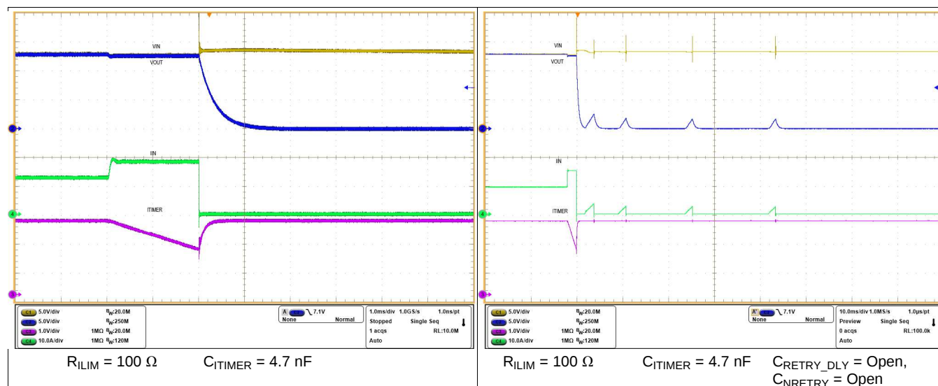
图 36. Circuit Breaker - Auto-Retry
