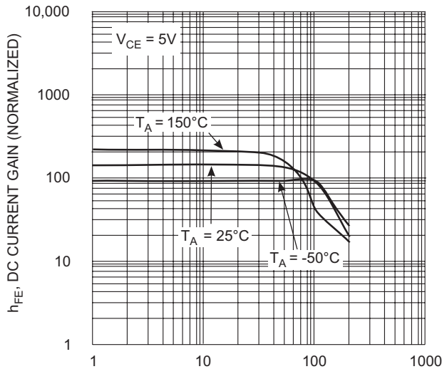
I_C , COLLECTOR CURRENT (mA) Fig. 7. DC Current Gain vs. Collector Current (PNP5401)
