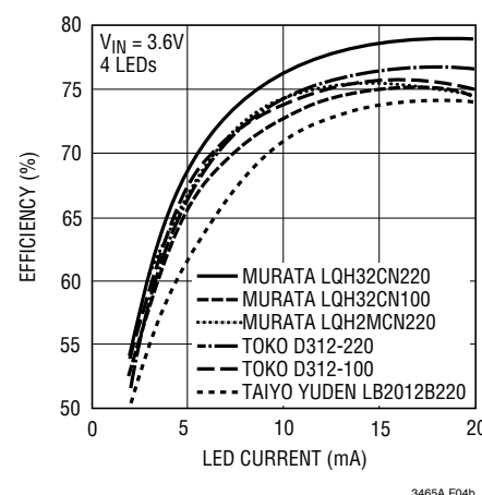
Figure 4b. Efficiency Comparison of Different Inductors (LT3465A)
