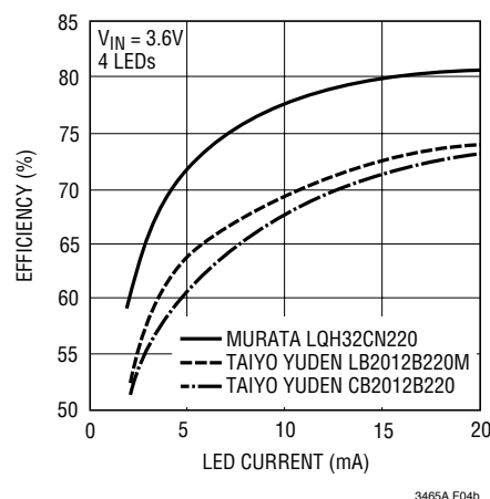
Figure 4a. Efficiency Comparison of Different Inductors (LT3465)
