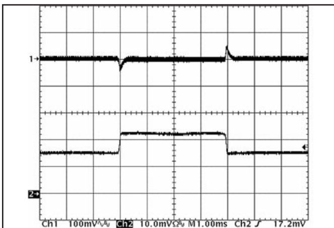
Figure 11: Output voltage response to step-change in load current (50%-75%-50% of I_{out(max)} ; dI/dt = 0.1A/\mu s ). Load cap: 15 \mu F, 450 m \Omega ESR tantalum capacitor and 1 \mu F ceramic capacitor. Top trace: V_{out} (100mV/div), Bottom trace: I_{out} (10A/div).
