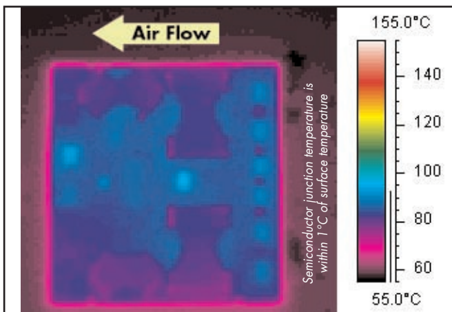
Figure 6: Thermal plot of converter at 30 amp load current with 55°C air flowing at the rate of 200 LFM. Air is flowing across the converter from output to input (nominal input voltage).
