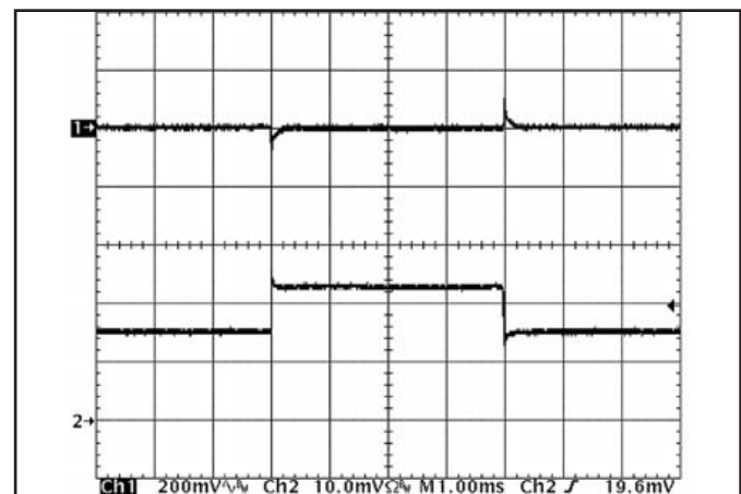
Figure 12: Output voltage response to step-change in load current (50%-75%-50% of I_{out(max)} ; dI/dt = 5A/\mu s ). Load cap: 480 \mu F, 15 m \Omega ESR tantalum capacitor and 1 \mu F ceramic capacitor. Top trace: V_{out} (200mV/div), Bottom trace: I_{out} (10A/div).
