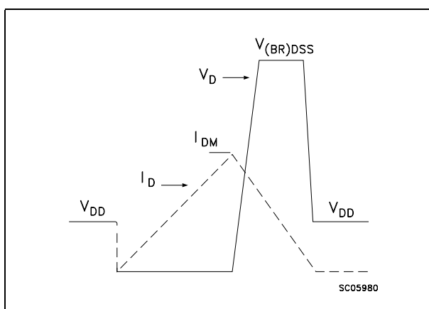
Figure 14. Unclamped inductive waveform
