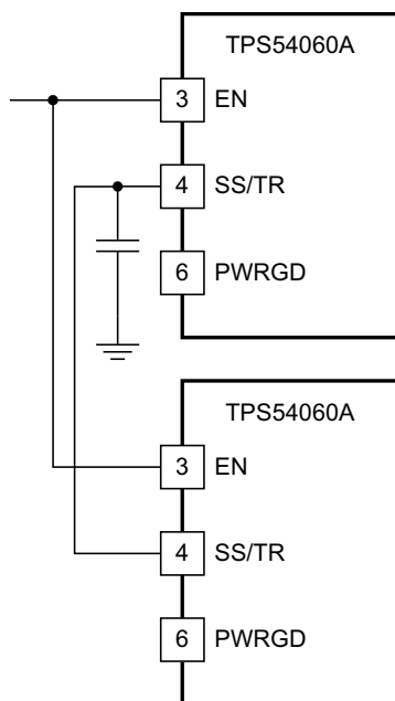
Figure 34. Schematic for Ratio-Metric Start-Up Sequence
