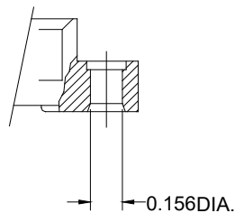
VARIATION 04 .156 +.002 DIA. MOUNTING HOLE -.000
