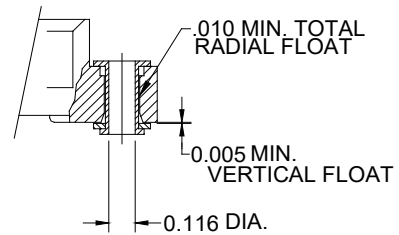
VARIATION 03 .116 +.003 I.D. FLOATING EYELET -.000
